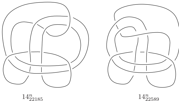
FIGURE 2. The genus two mutant pair K_0 = 14^n_{22185} and K_0^\tau = 14^n_{22589} .
