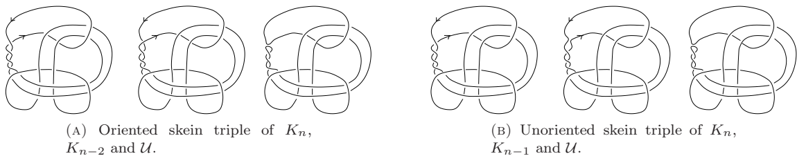
FIGURE 4. Oriented and unoriented skein triples.
