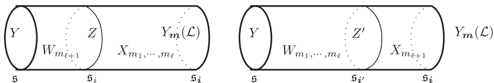
Fig. 4. Two different decompositions of the two-handle cobordism W_{m_1, \dots, m_{\ell+1}} from Y to Y_{\mathbf{m}}(\mathcal{L}) used in Lemma 5.10. The left cobordism consists of first attaching the two-handle to L_{\ell+1} and then attaching the remaining two-handles. The right cobordism consists of first attaching the two-handles along all components other than L_{\ell+1} and then attaching a two-handle along L_{\ell+1} .
